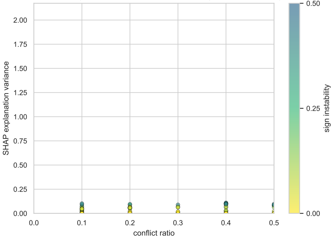
cat__protocol_type_tcp: SHAP explanation variance (Spearman r = 0.142)
